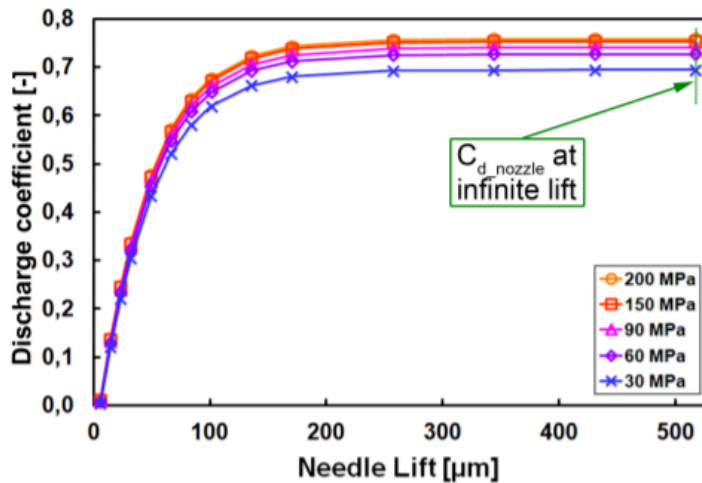
Figure 53: Relation between needle lift and discharge coefficient used by Tol
