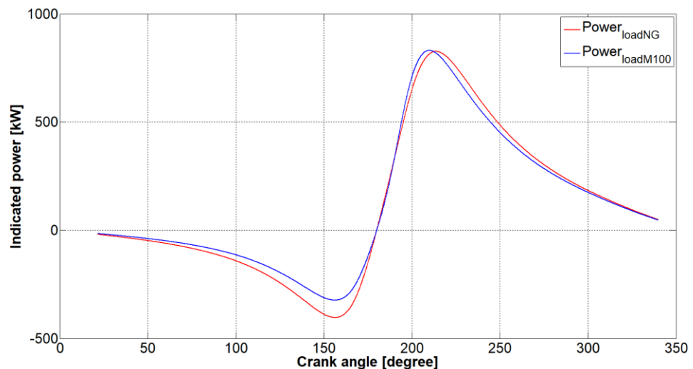
Figure 32: Indicated power plot of cylinder 4 for NG compared to methanol at 375 kW e
