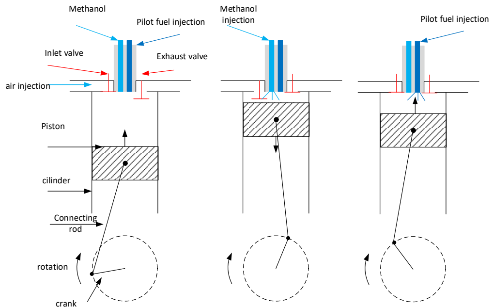
Figure 13: Schematic overview of the direct injection of methanol and separate pilot fuel
